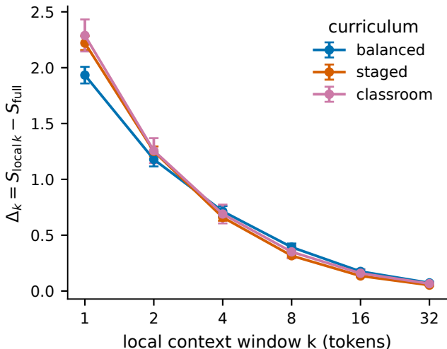
Surprisal degradation under context truncation
